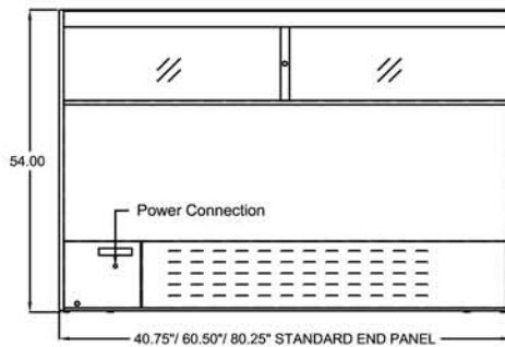
PLAN & REAR VIEW
