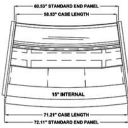
B - Server Side KD15INT = 72.11"
