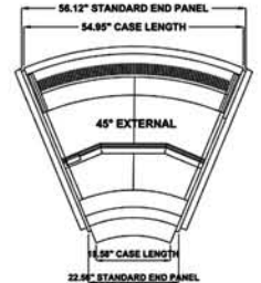
B - Server Side KD45EXT = 22.56"
