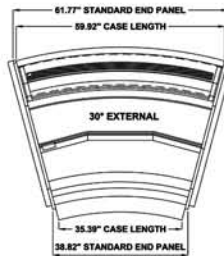
B - Server Side KD30EXT = 38.82"
