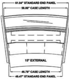
B - Server Side KD15EXT = 49.47"
