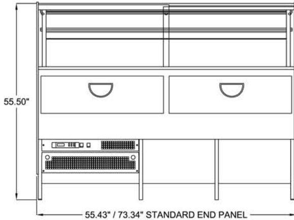
PLAN & REAR VIEW
