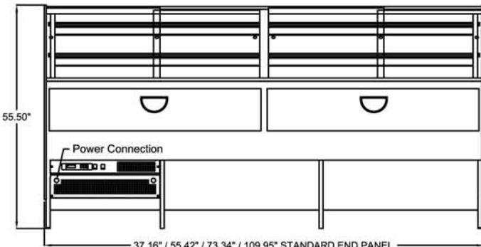
37.16" / 55.42" / 73.34" / 109.95" STANDARD END PANEL
